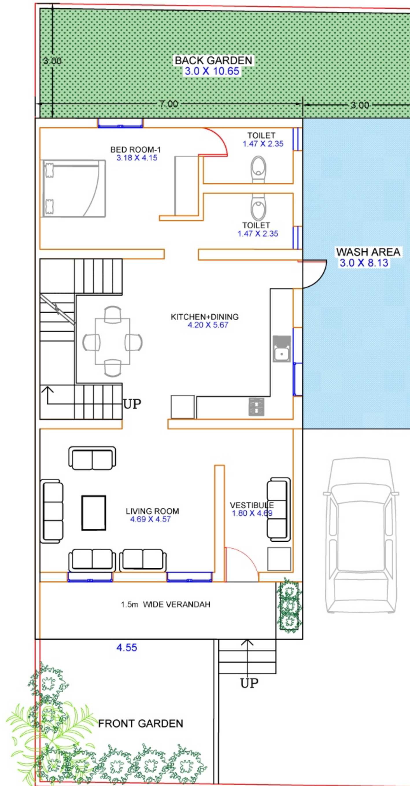
GROUND FLOOR
