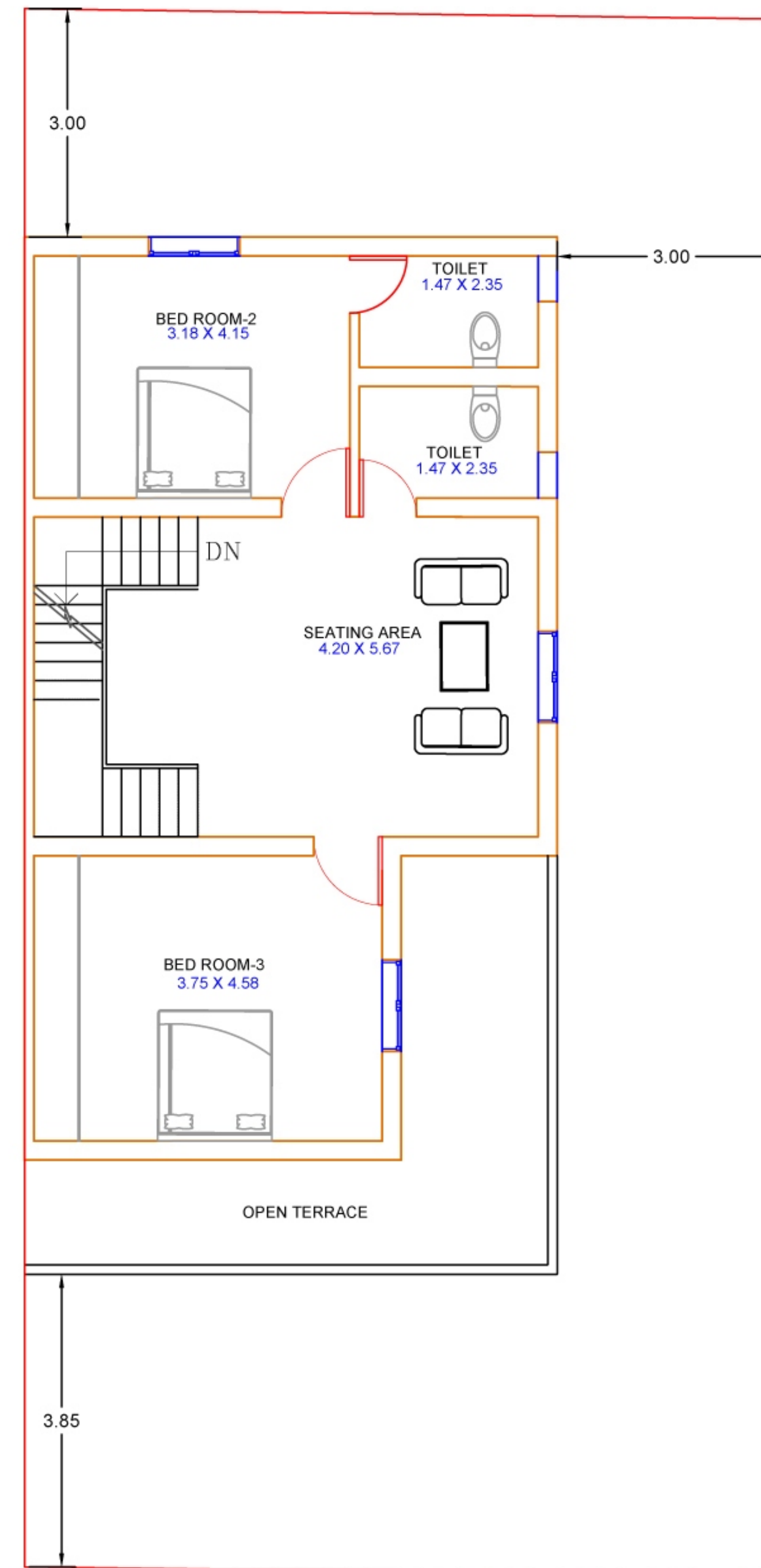
FIRST FLOOR
